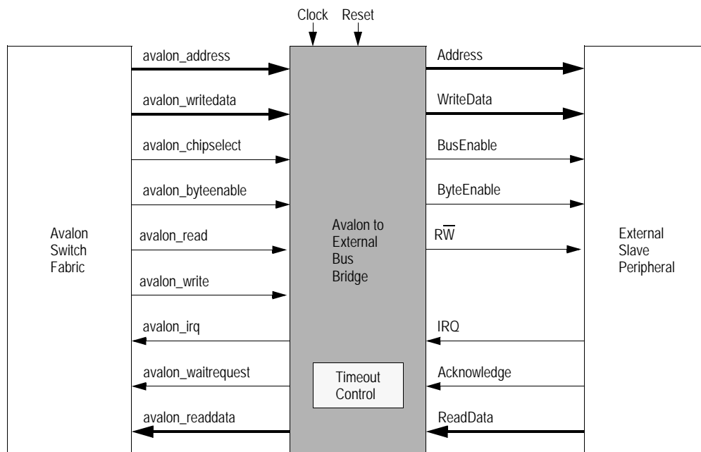
Figure 1. Avalon to External Bus Bridge Block Diagram
